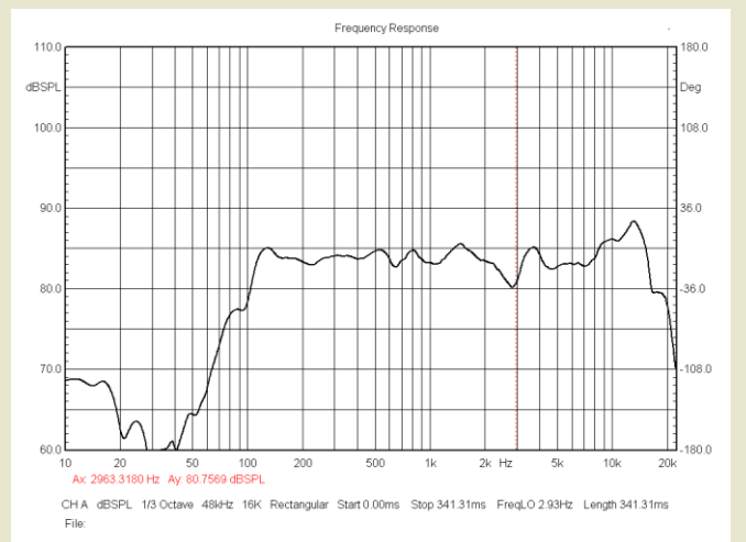
Frequency Response ( \pm 3\% )_MF 10
